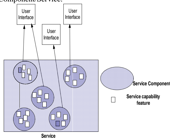
Figure 7 : service decomposition in a service provider view
